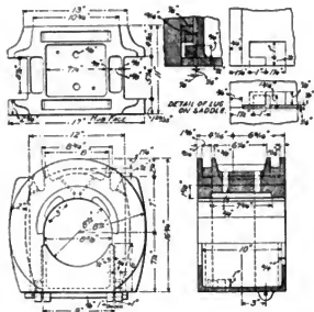
Figs. 1431-1436. Cast-Steel Driving Box for Journals 8 1/4 in. x 11 in.
